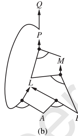
Figure 7.16 (a) A set of Horn clauses. (b) The corresponding AND-OR graph.
