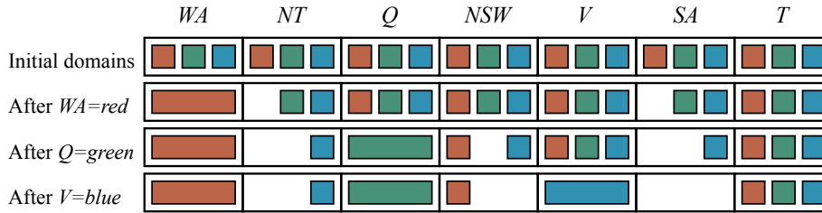
Figure 5.7 The progress of a map-coloring search with forward checking. WA = red is assigned first; then forward checking deletes red from the domains of the neighboring variables NT and SA . After Q = green is assigned, green is deleted from the domains of NT , SA , and NSW . After V = blue is assigned, blue is deleted from the domains of NSW and SA , leaving SA with no legal values.
