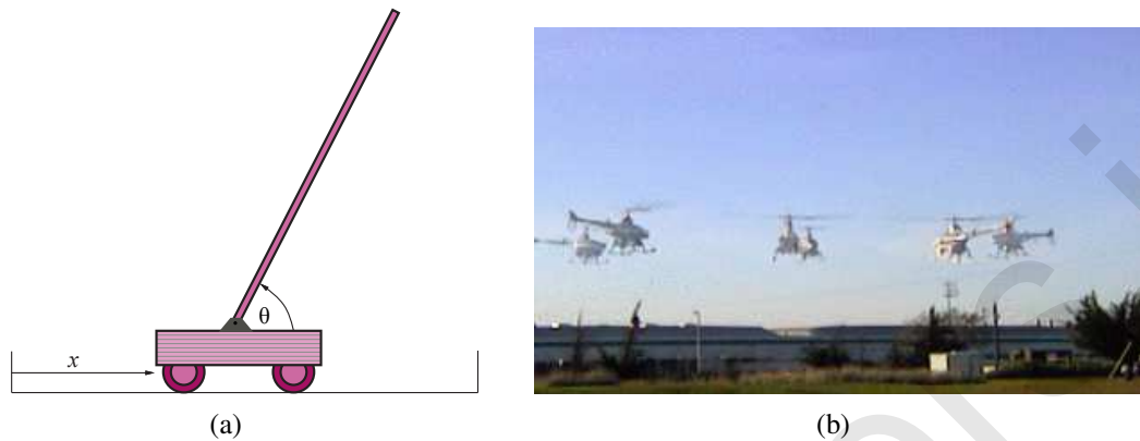
Figure 23.9 (a) Setup for the problem of balancing a long pole on top of a moving cart. The cart can be jerked left or right by a controller that observes the cart’s position x and velocity \dot{x} , as well as the pole’s angle \theta and rate of change of angle \dot{\theta} . (b) Six superimposed time-lapse images of a single autonomous helicopter performing a very difficult “nose-in circle” maneuver. The helicopter is under the control of a policy developed by the PEGASUS policy-search algorithm (Ng et al. , 2003). A simulator model was developed by observing the effects of various control manipulations on the real helicopter; then the algorithm was run on the simulator model overnight. A variety of controllers were developed for different maneuvers. In all cases, performance far exceeded that of an expert human pilot using remote control. (Image courtesy of Andrew Ng.)
