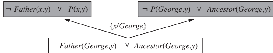
Figure 20.14 An inverse resolution step that generates a new predicate P .
