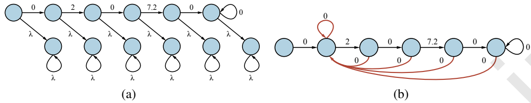
Figure 16.13 (a) The reward sequence M = 0, 2, 0, 7.2, 0, 0, \dots augmented with a choice to switch permanently to a constant arm M_\lambda at each point. (b) An MDP whose optimal value is exactly equivalent to the optimal value for (a), at the point where the optimal policy is indifferent between M and M_\lambda .
