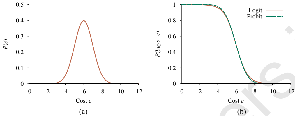
Figure 13.8 (a) A normal (Gaussian) distribution for the cost threshold, centered on \mu=6.0 with standard deviation \sigma=1.0 . (b) Expit and probit models for the probability of buys given cost , for the parameters \mu=6.0 and \sigma=1.0 .
