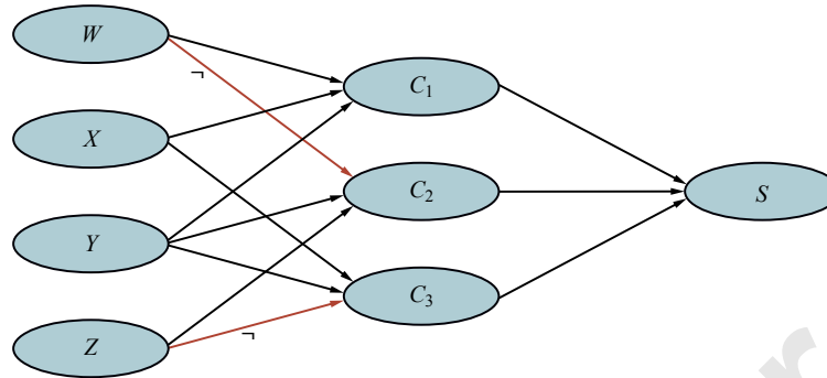
Figure 13.14 Bayes net encoding of the 3-CNF sentence
