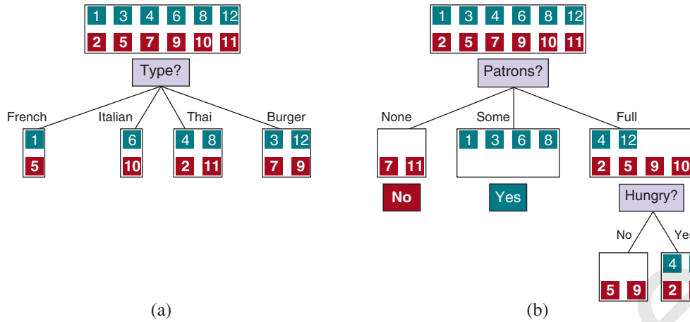
Figure 19.4 Splitting the examples by testing on attributes. At each node we show the positive (light boxes) and negative (dark boxes) examples remaining. (a) Splitting on Type brings us no nearer to distinguishing between positive and negative examples. (b) Splitting on Patrons does a good job of separating positive and negative examples. After splitting on Patrons , Hungry is a fairly good second test.
