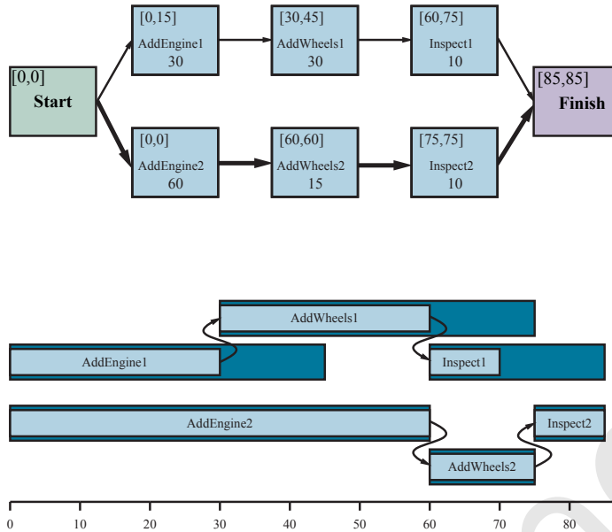
Figure 11.14 Top: a representation of the temporal constraints for the job-shop scheduling problem of Figure 11.13. The duration of each action is given at the bottom of each rectangle. In solving the problem, we compute the earliest and latest start times as the pair [ES, LS] , displayed in the upper left. The difference between these two numbers is the slack of an action; actions with zero slack are on the critical path, shown with bold arrows. Bottom: the same solution shown as a timeline. Blue rectangles represent time intervals during which an action may be executed, provided that the ordering constraints are respected. The unoccupied portion of a blue rectangle indicates the slack.
