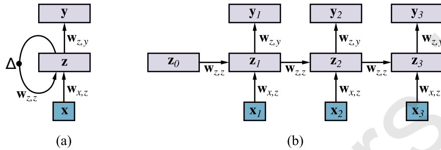
Figure 22.8 (a) Schematic diagram of a basic RNN where the hidden layer \mathbf{z} has recurrent connections; the \Delta symbol indicates a delay. (b) The same network unrolled over three time steps to create a feedforward network. Note that the weights are shared across all time steps.
