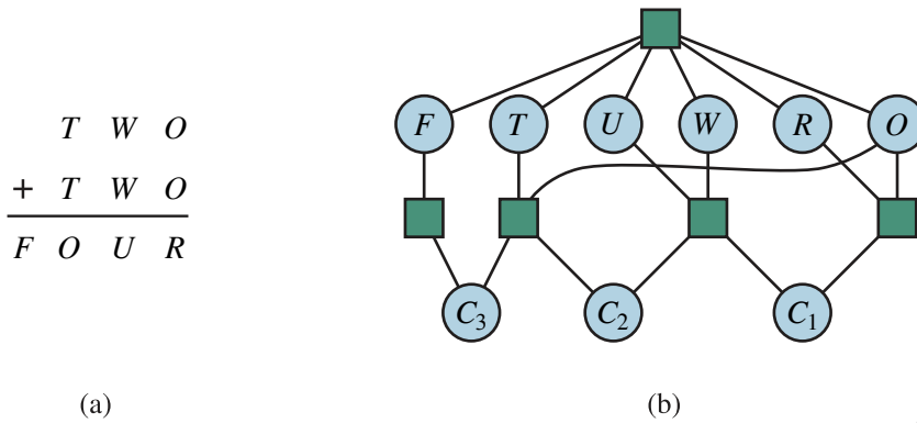
Figure 5.2 (a) A cryptarithmic problem. Each letter stands for a distinct digit; the aim is to find a substitution of digits for letters such that the resulting sum is arithmetically correct, with the added restriction that no leading zeroes are allowed. (b) The constraint hypergraph for the cryptarithmic problem, showing the Alldiff constraint (square box at the top) as well as the column addition constraints (four square boxes in the middle). The variables C_1 , C_2 , and C_3 represent the carry digits for the three columns from right to left.
