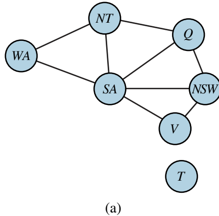
Figure 9.5 (a) Constraint graph for coloring the map of Australia. (b) The map-coloring CSP expressed as a single definite clause. Each map region is represented as a variable whose value can be one of the constants Red , Green , or Blue (which are declared Diff ).
