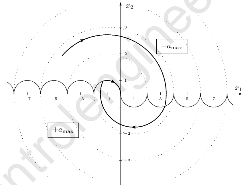
Fig. S.1. Optimal feedback control law for the time-optimal motion.
