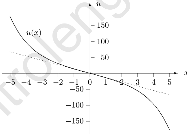
Fig. 3.3. Approximately optimal controller for a = 3 , q = 100 .
