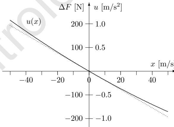
Fig. 3.4. Characteristic of the LQQ controller for v_0 = 100 m/s and q = 0.001 with c_w = 0.05 , A_r = 0.5 m 2 , \rho = 1.3 kg/m 3 , and m = 200 kg.
