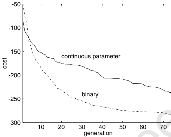
Figure 4.19 Convergence of the binary and continuous parameter GAs as a function of generation when averaged over ten different runs.
