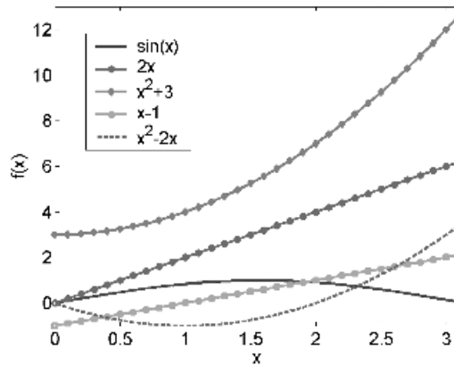
Figure 7.13 Plots of chromosomes approximating \sin(x) .
