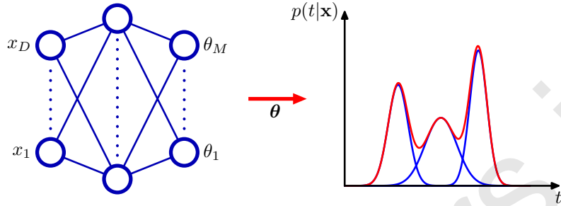
Figure 5.20 The mixture density network can represent general conditional probability densities p(t|\mathbf{x}) by considering a parametric mixture model for the distribution of t whose parameters are determined by the outputs of a neural network that takes \mathbf{x} as its input vector.
