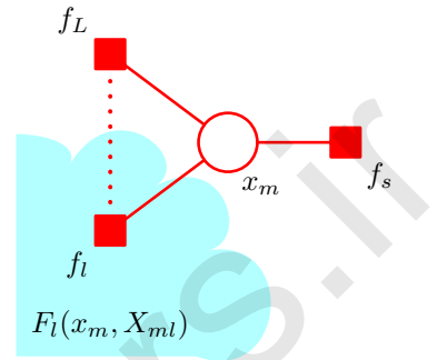
Figure 8.48 Illustration of the evaluation of the message sent by a variable node to an adjacent factor node.
