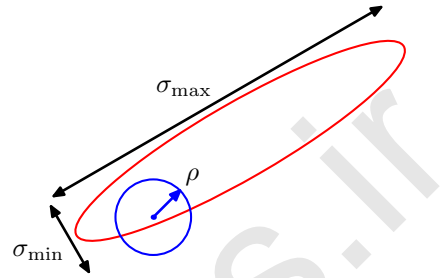
Figure 11.10 Schematic illustration of the use of an isotropic Gaussian proposal distribution (blue circle) to sample from a correlated multivariate Gaussian distribution (red ellipse) having very different standard deviations in different directions, using the Metropolis-Hastings algorithm. In order to keep the rejection rate low, the scale \rho of the proposal should be on the order of the smallest standard deviation \sigma_{\min} , which leads to random walk behaviour in which the number of steps separating states that are approximately independent is of order (\sigma_{\max}/\sigma_{\min})^2 where \sigma_{\max} is the largest standard deviation.
