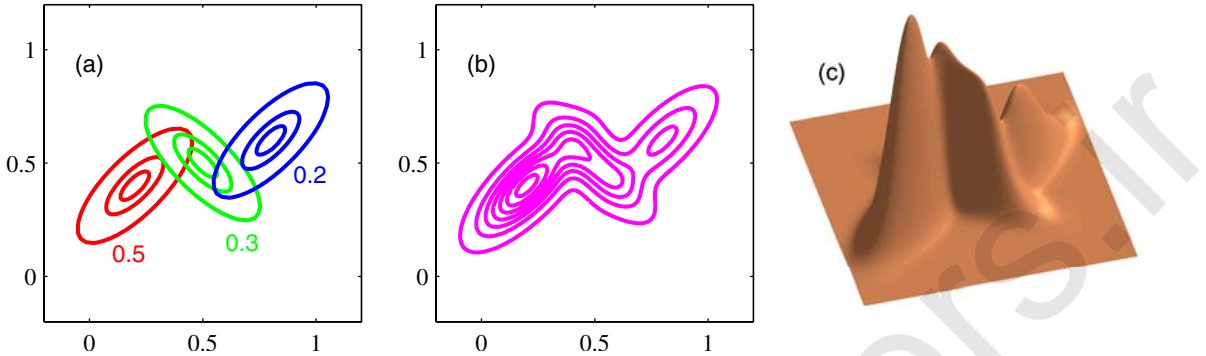
Figure 2.23 Illustration of a mixture of 3 Gaussians in a two-dimensional space. (a) Contours of constant density for each of the mixture components, in which the 3 components are denoted red, blue and green, and the values of the mixing coefficients are shown below each component. (b) Contours of the marginal probability density p(\mathbf{x}) of the mixture distribution. (c) A surface plot of the distribution p(\mathbf{x}) .
