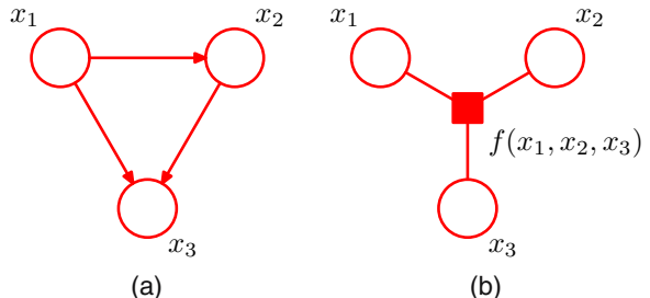
Figure 8.44 (a) A fragment of a directed graph having a local cycle. (b) Conversion to a fragment of a factor graph having a tree structure, in which f(x_1, x_2, x_3) = p(x_1)p(x_2|x_1)p(x_3|x_1, x_2) .
