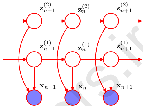
Figure 13.19 A factorial hidden Markov model comprising two Markov chains of latent variables. For continuous observed variables x , one possible choice of emission model is a linear-Gaussian density in which the mean of the Gaussian is a linear combination of the states of the corresponding latent variables.
