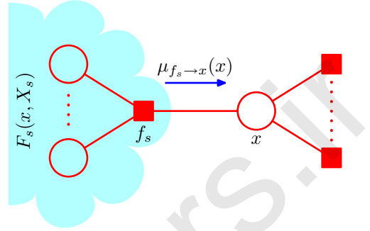
Figure 8.46 A fragment of a factor graph illustrating the evaluation of the marginal p(x) .
