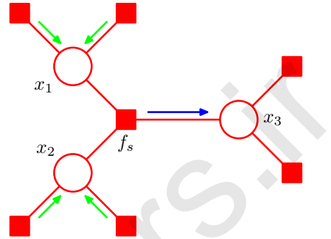
Figure 8.50 The sum-product algorithm can be viewed purely in terms of messages sent out by factor nodes to other factor nodes. In this example, the outgoing message shown by the blue arrow is obtained by taking the product of all the incoming messages shown by green arrows, multiplying by the factor f_s , and marginalizing over the variables x_1 and x_2 .
