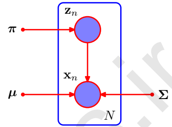
Figure 9.9 This shows the same graph as in Figure 9.6 except that we now suppose that the discrete variables z_n are observed, as well as the data variables x_n .
