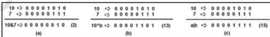
Figure 2.2. (a) Result of the AND operator. (b) Result of the EXCLUSIVE OR operator. (c) Result of the OR operator.
