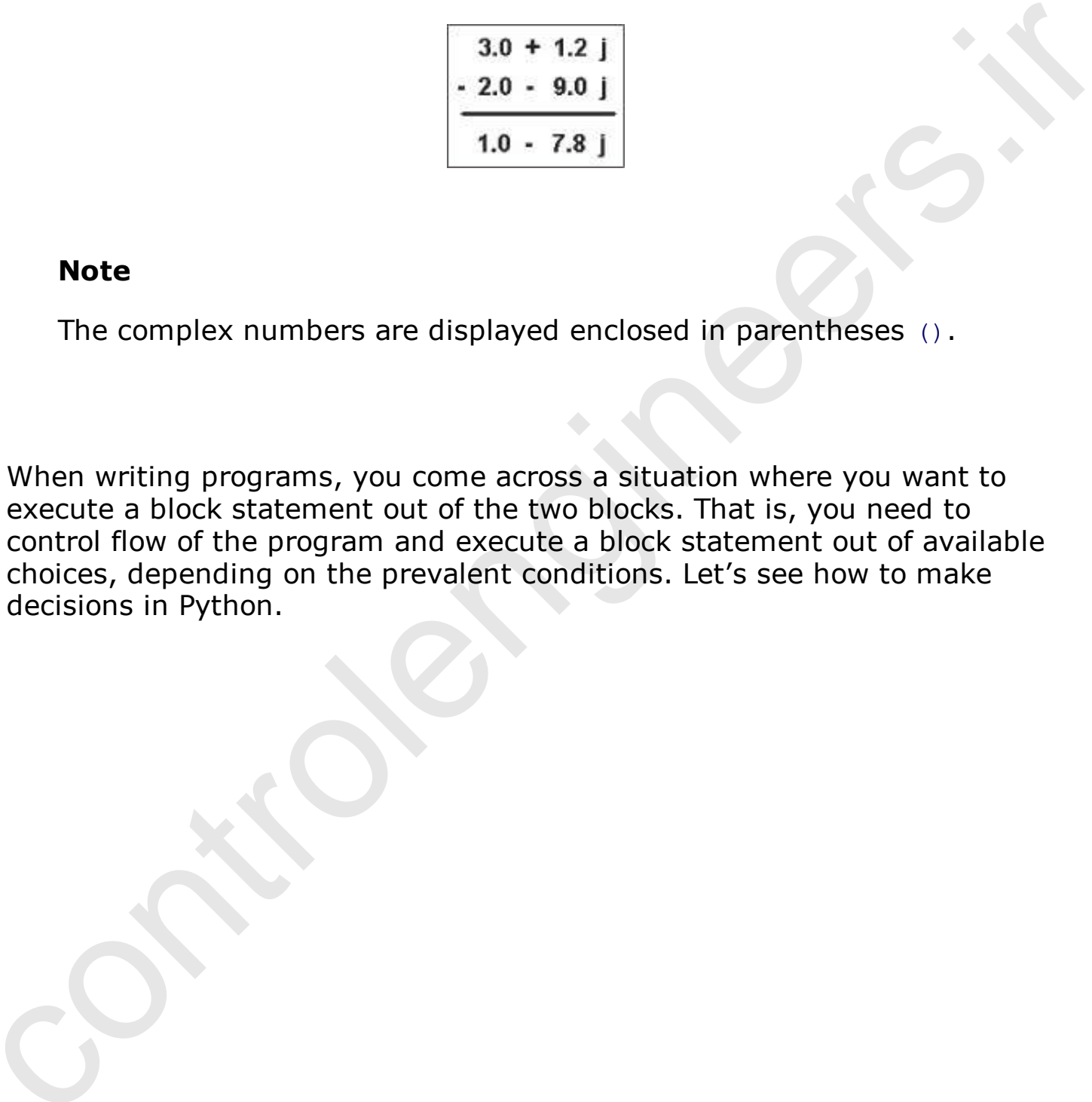
Figure 2.4. Addition of two complex numbers.
